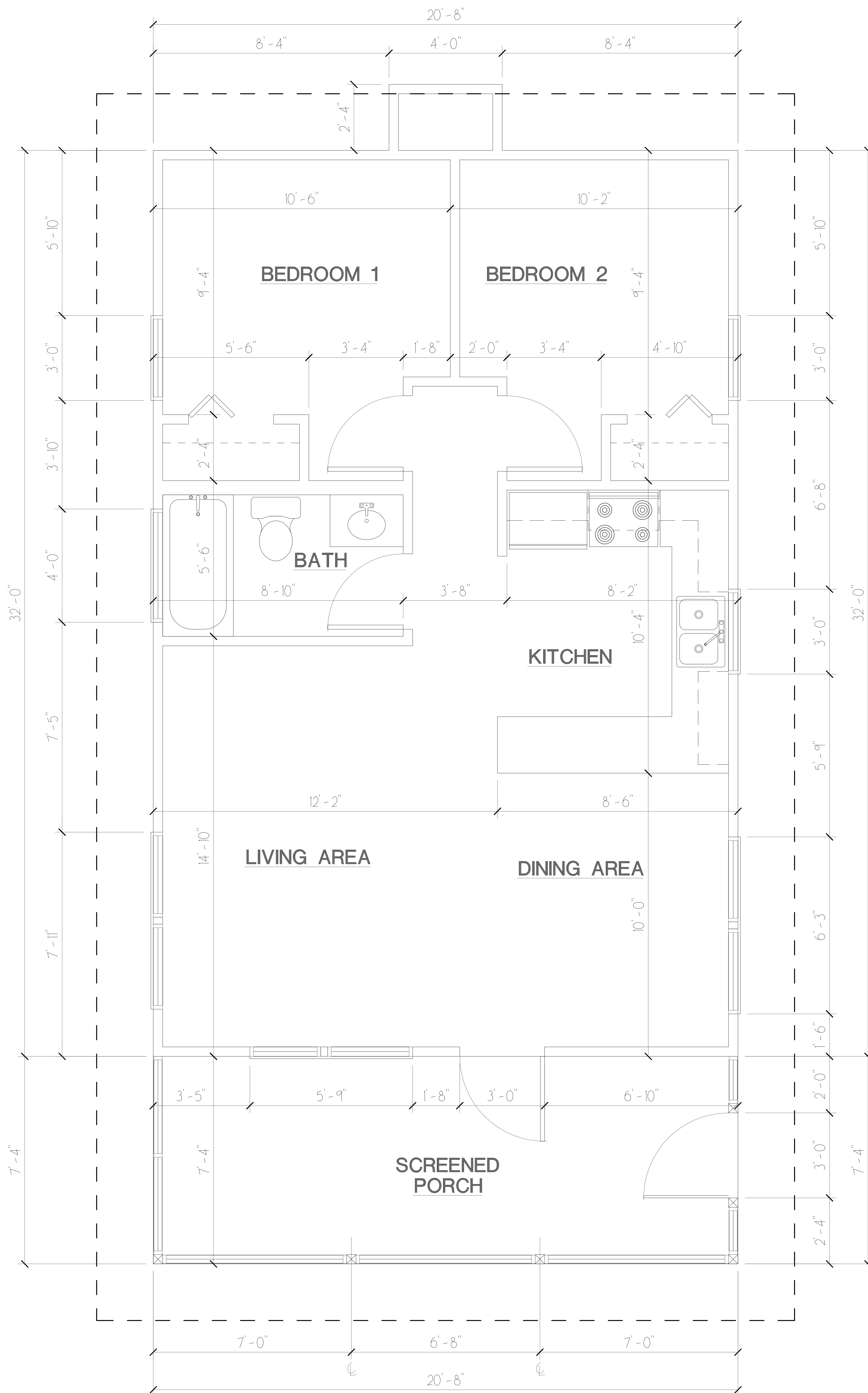
FLOOR PLAN – UNIT 'A'
