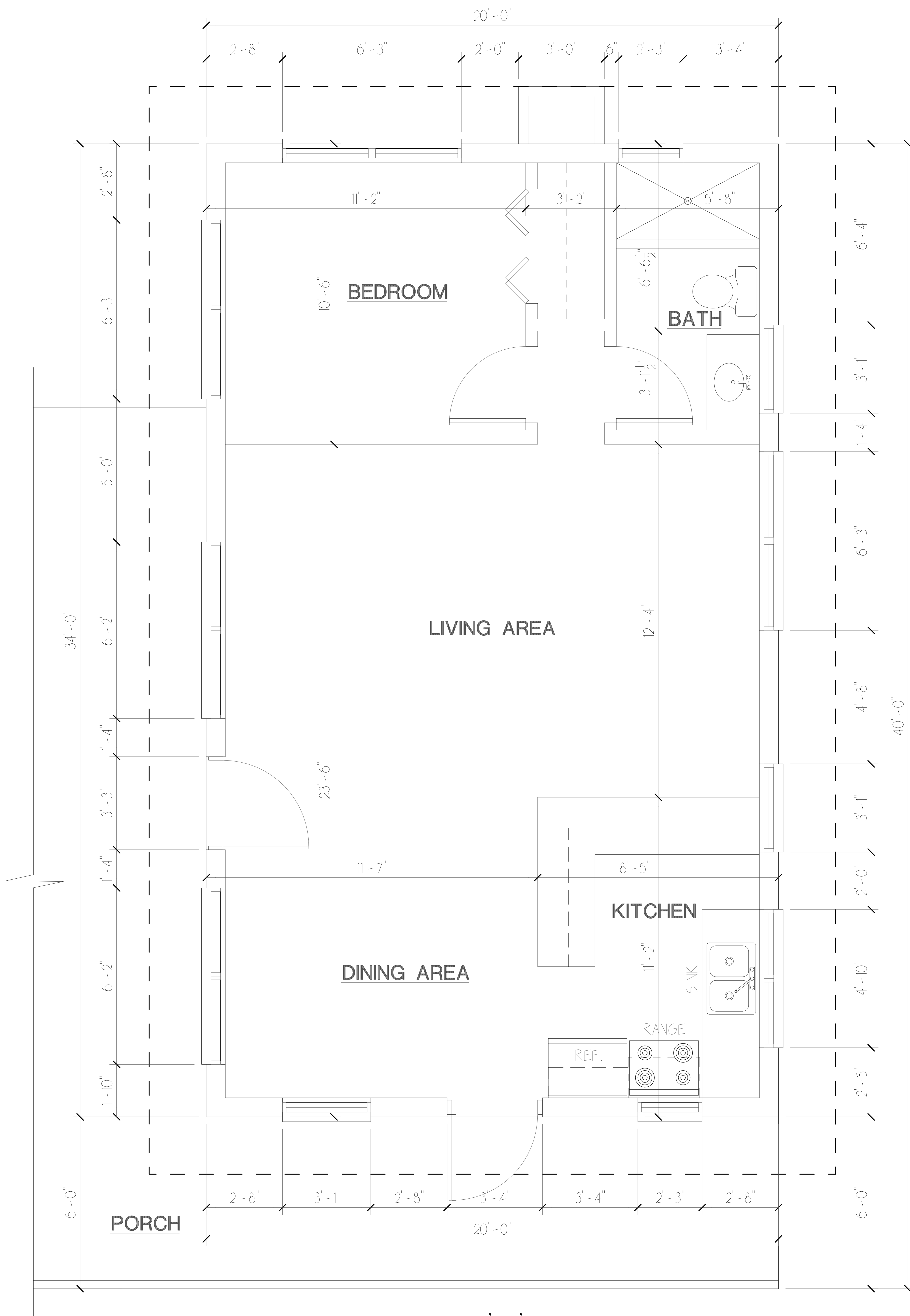
FLOOR PLAN – UNIT 'C'
