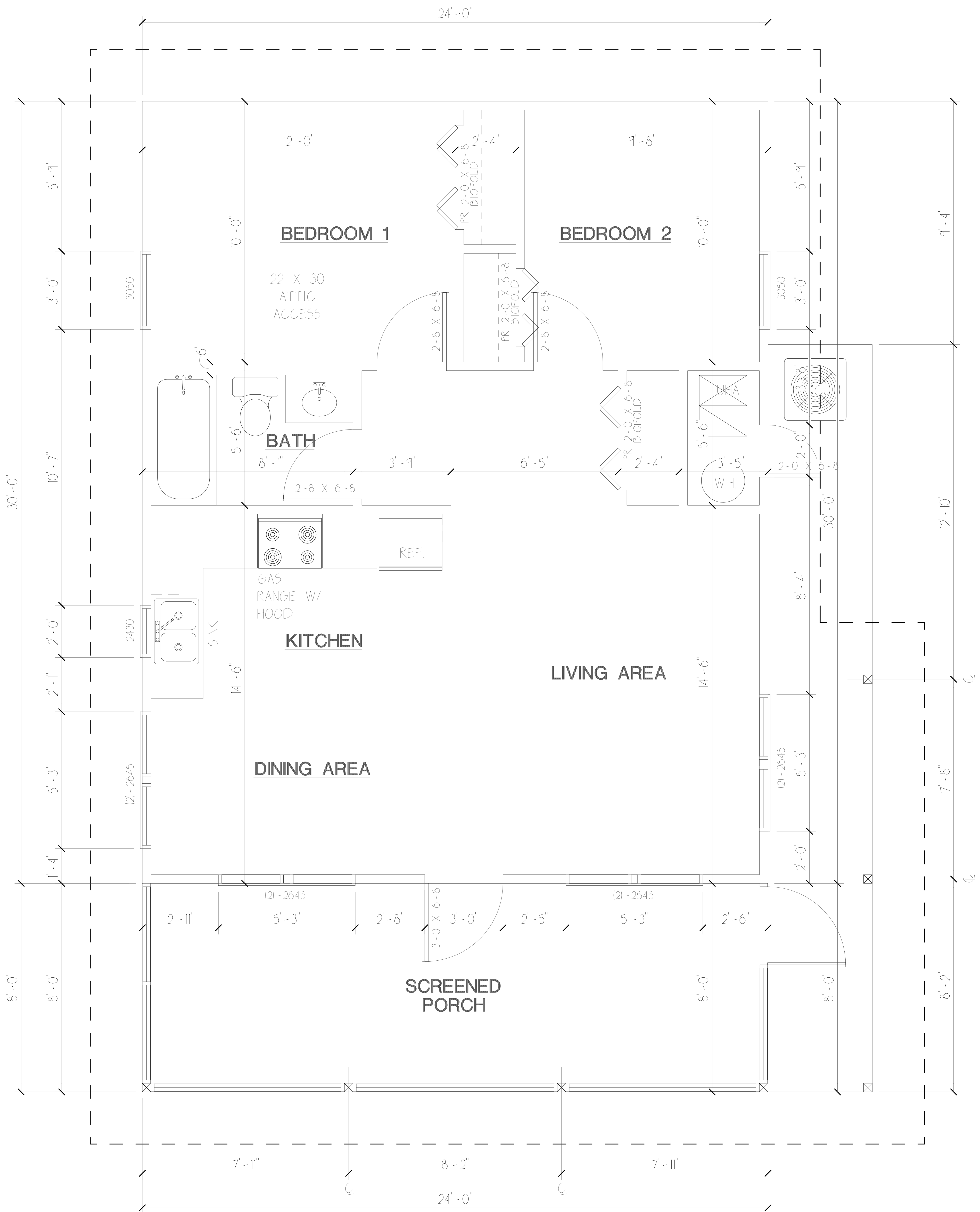
FLOOR PLAN – UNIT 'B' NTS
